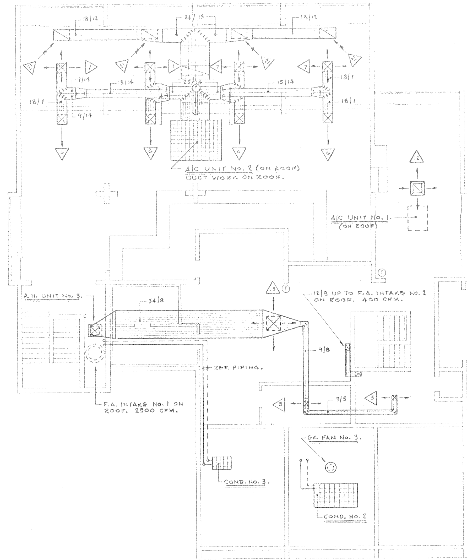
2nd FLOOR PLAN 1/8" = 1'-0"
